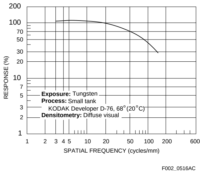
Modulation-Transfer Curve
