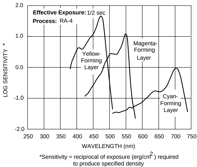
Spectral-Sensitivity Curves
