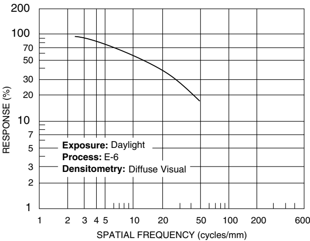
Modulation-Transfer Curves
