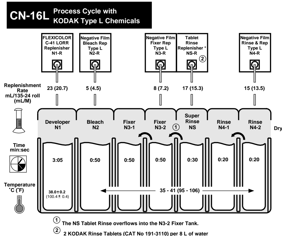
Figure 1 Specifications for Process CN-16L
