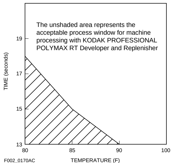
Machine Process Window Time and Temperature
