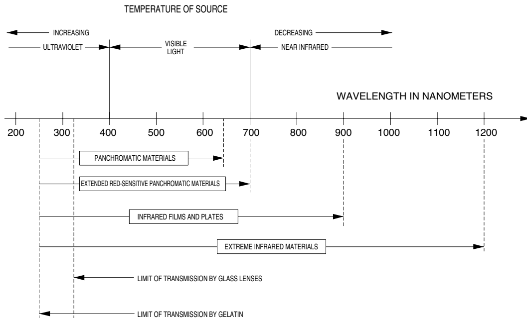
Figure 1: Spectral Range of Radiation Recording Methods
